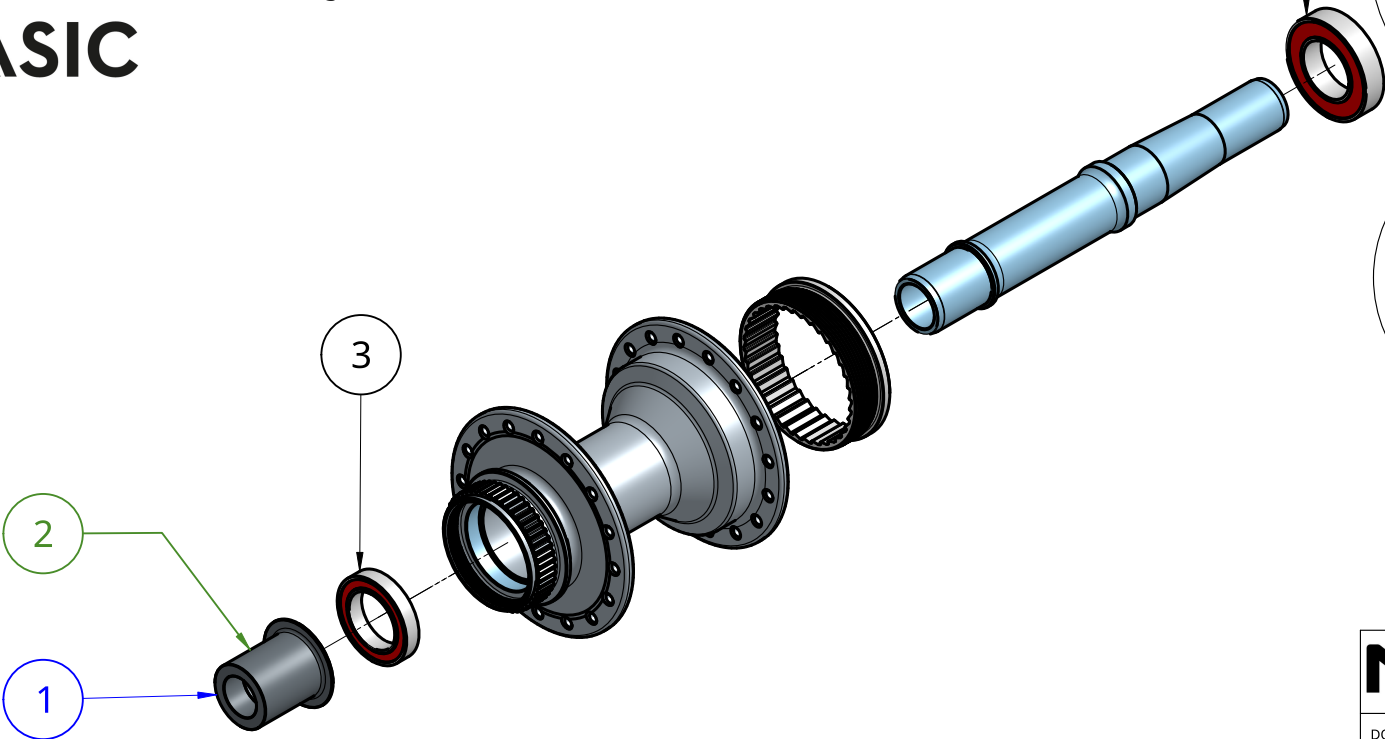
detailed freewheel explode sheet 3
